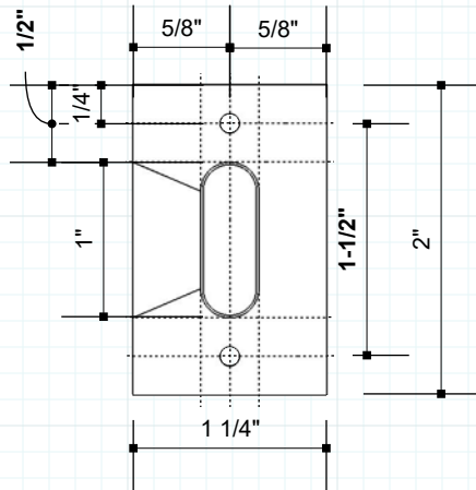
Catch Plate
